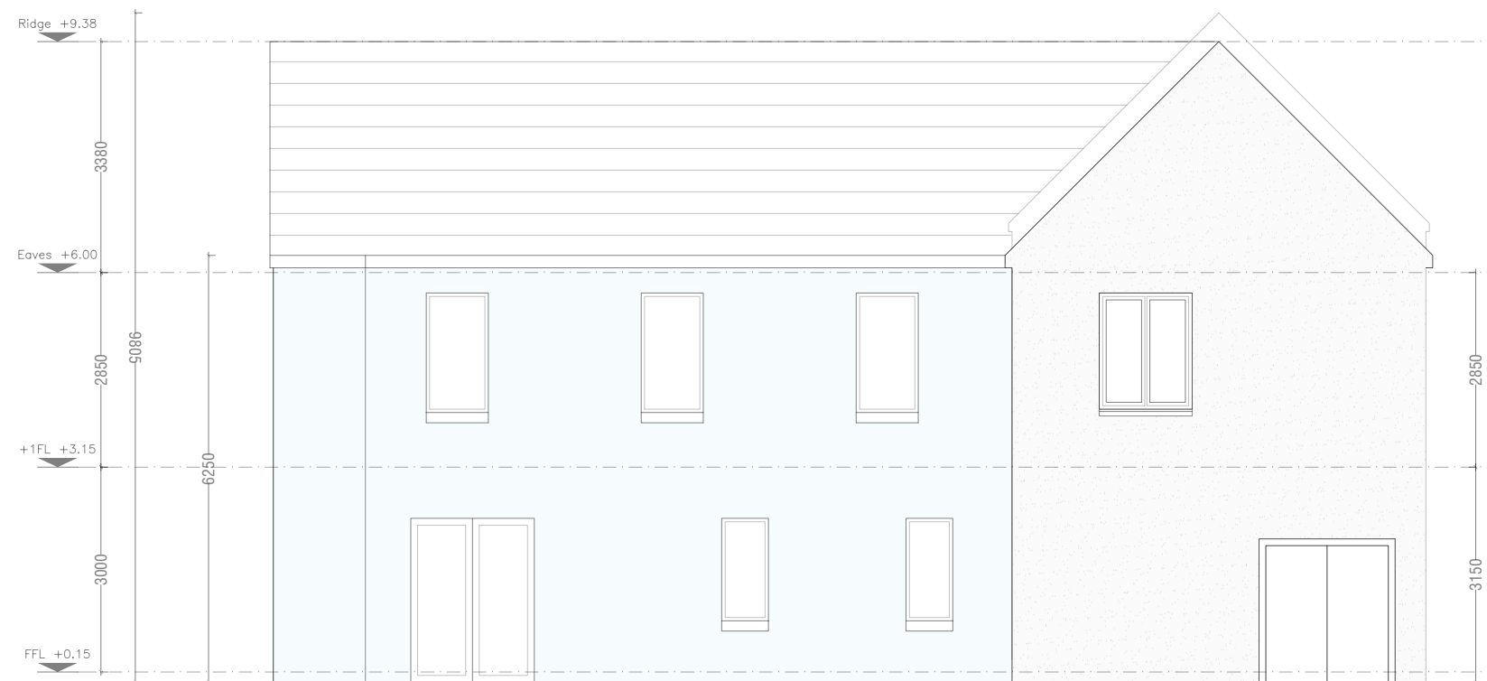
Creche Rear Elevation (North)
